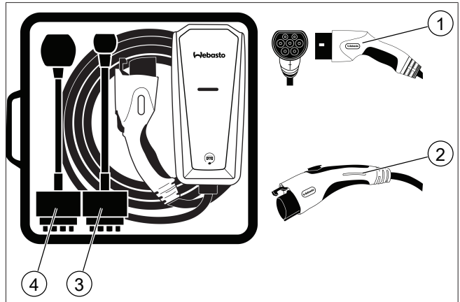
Fig. 5 Webasto Go Mobile Charger
