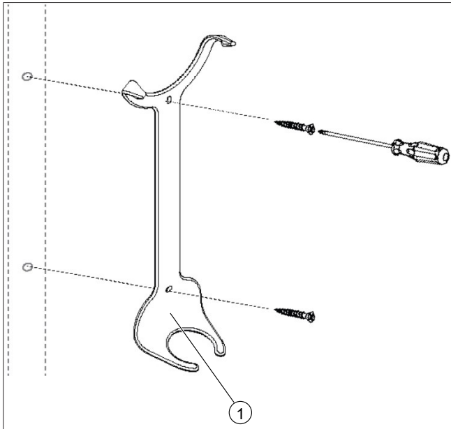
Fig. 6 Wall hanger
