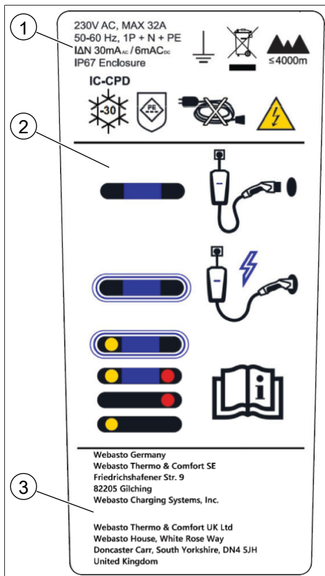
Fig. 3 Label CCID Caution EU and UK Webasto
