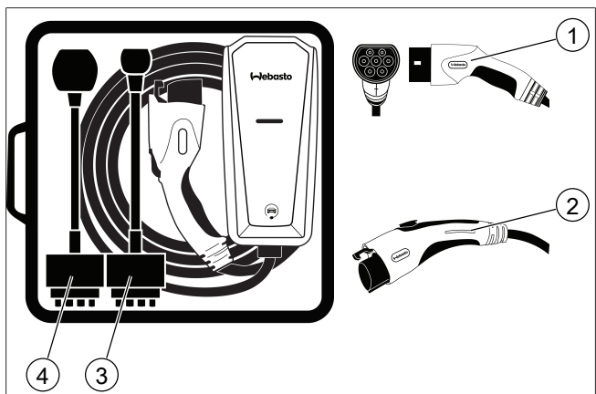
Fig. 8 Webasto Go Mobile Charger
